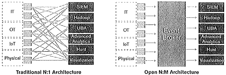
Traditional N:1 Architecture Open N:M Architecture Figure 4. Intelligent message bus architecture
